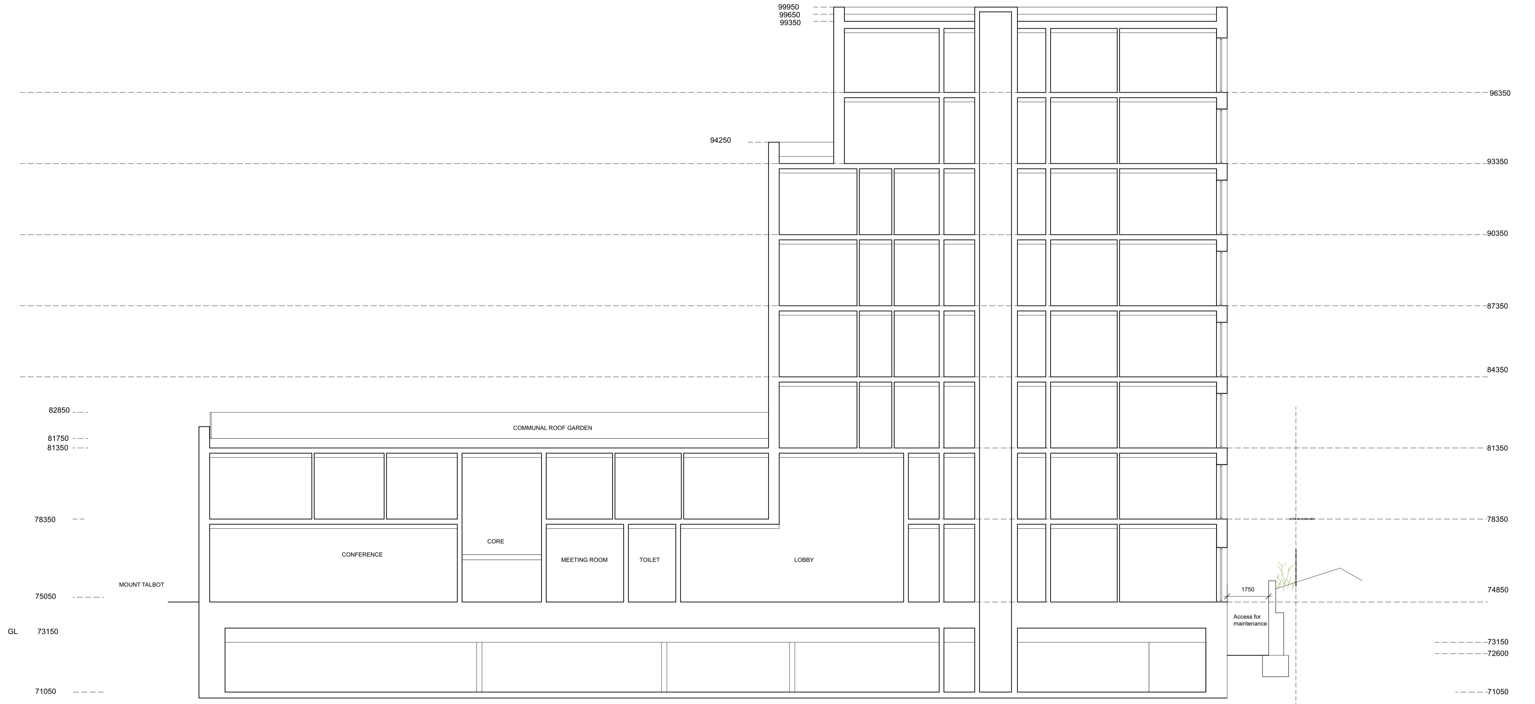
SECTION CC
