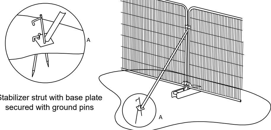
Stabilizer struts installed on every fencing panel section on the tree protection side
