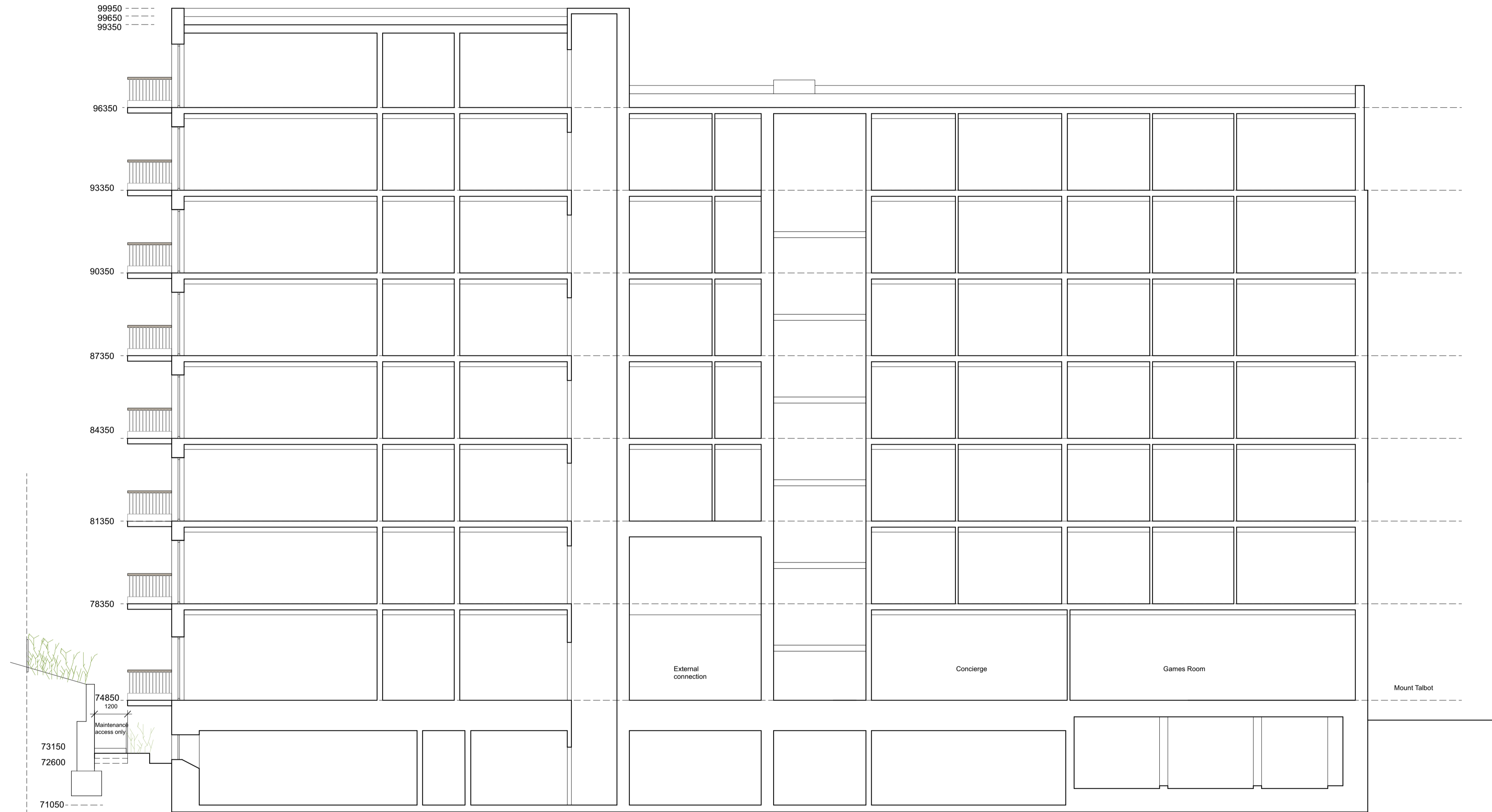
SECTION EE
