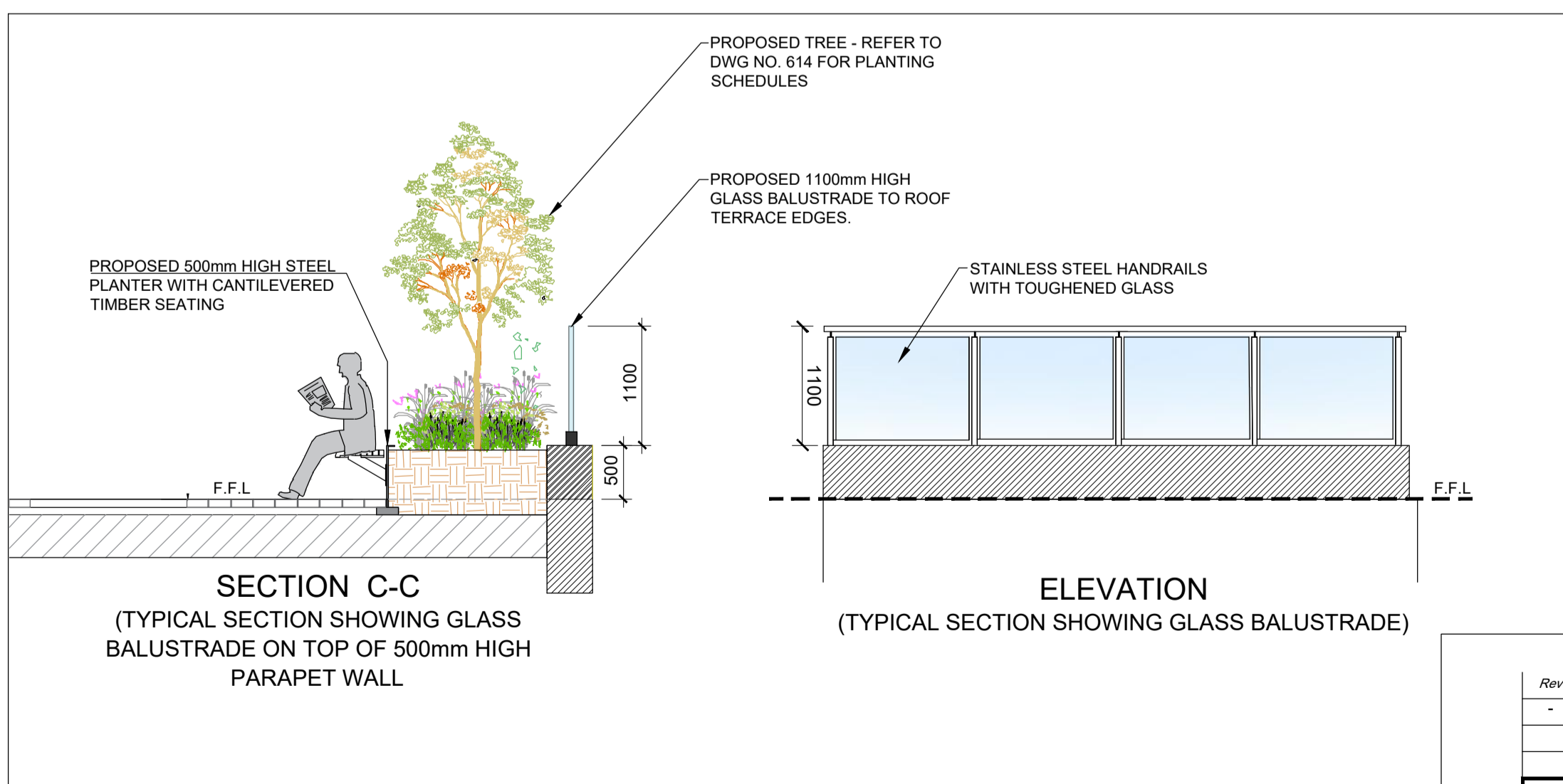
PROPOSED 850mm / 1000mm HIGH GALVANIZED STEEL RAILING DETAIL - 1:50
